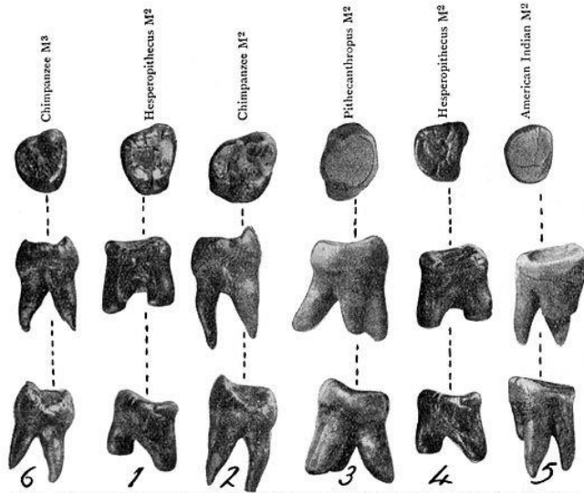
FIG. 2.—Comparison of the Second Superior Molars of the Right Side of the Upper Jaw in the Primates. Upper row : crown views of the superior molars. Middle row : anterior views of the same teeth. Lower row : posterior views of the same teeth. (1) Hesperopithecus, the new Nebraska Primate, middle-aged. (2) Anthropopithecus, a young chimpanzee. (3) Pithecanthropus, adult Trinil Ape-man. (4) Hesperopithecus (photographed in a different light). (5) Homo sapiens mongoloides , aged North American Indian. (6) Third superior molar of Anthropopithecus, a young chimpanzee All photographed to the same scale and natural size.
